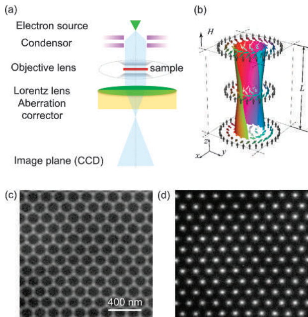
Fig. 1. (a) Schematic representation of the electron-optical elements used in Lorentz TEM. The objective lens is turned off to produce a magnetic-field-free condition at the position of the sample. (b) Magnetic configuration of a Bloch-type skyrmion in a thin film of thickness L and in the presence of H magnetic field. (c) Underfocus and (d) overfocus Fresnel images of a skyrmion lattice in an FeGe specimen formed in the presence of a 100 mT applied magnetic field at a temperature of 200 K. The images were recorded at defocus values of \pm 0.4 mm
