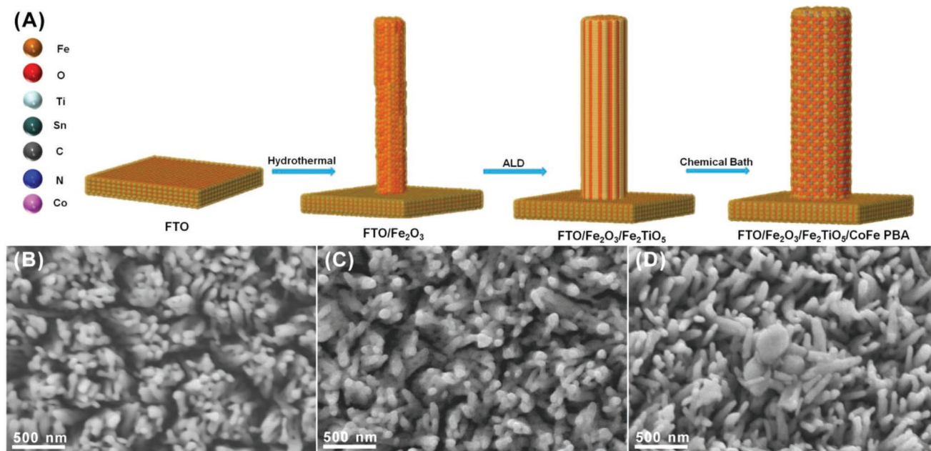
Figure 1. A) 3D Atomic supercell models with solvent accessible surface illustrating the synthetic procedure for \text{Fe}_2\text{O}_3/\text{Fe}_2\text{TiO}_5/\text{CoFe PBA} photoanodes. SEM images of B) \text{Fe}_2\text{O}_3 , C) \text{Fe}_2\text{O}_3/\text{Fe}_2\text{TiO}_5 , and D) \text{Fe}_2\text{O}_3/\text{Fe}_2\text{TiO}_5/\text{CoFe PBA} electrodes.
