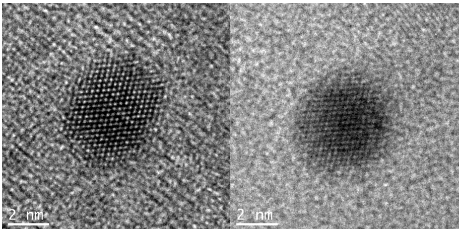
Figure 2. Image of Au particle supported on Al 2 O 3 recorded at 0.5mbar (left) and 5mbar (right) pressure of N 2 . The sample is a catalyst for methanol synthesis.
