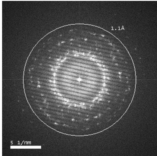
Figure 1. Youngs fringe experiment showing the resolution of the environmental Titan under 0.5mbar N 2 pressure. The fringes are easily recognized up to 9.2 nm -1 corresponding to 1.1 Å.
