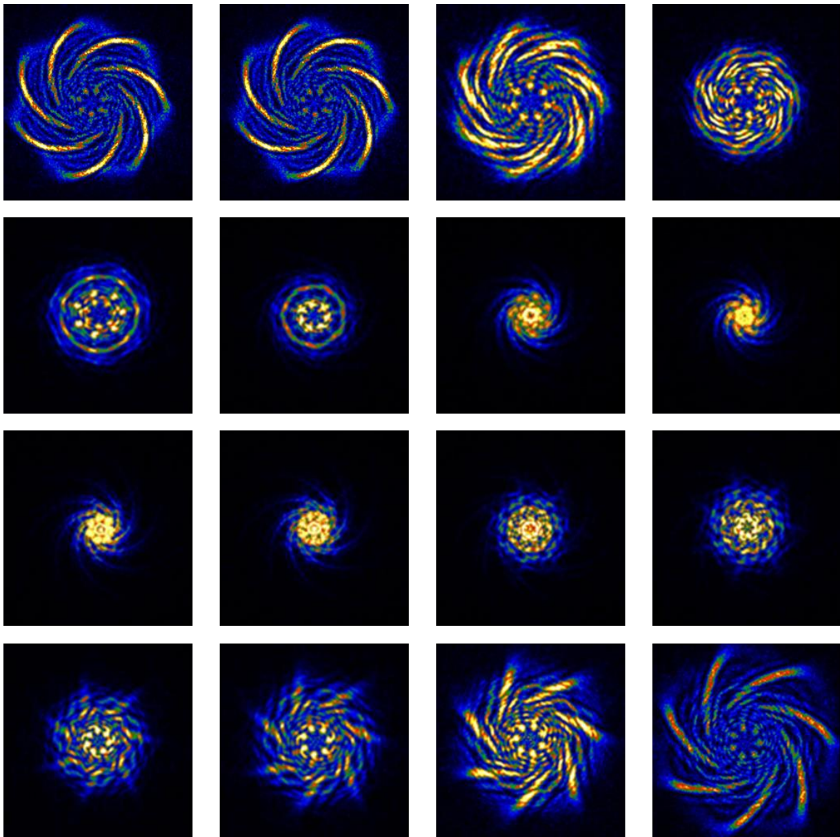
Fig. S1 Experimental defocus series for a logarithmic spiral. The apparent chirality changes with defocus.
