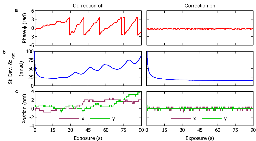
Fig. 3. Drift-corrected acquisition test (monitoring profiles). (a) Position of the fringes (in rad between +\pi and -\pi ), (b) standard deviation of the phase in the vacuum \delta\phi_{\text{vac}} and (c) lateral position of the sample ( x,y ) as a function of exposure time, without (left) and with correction (right).
