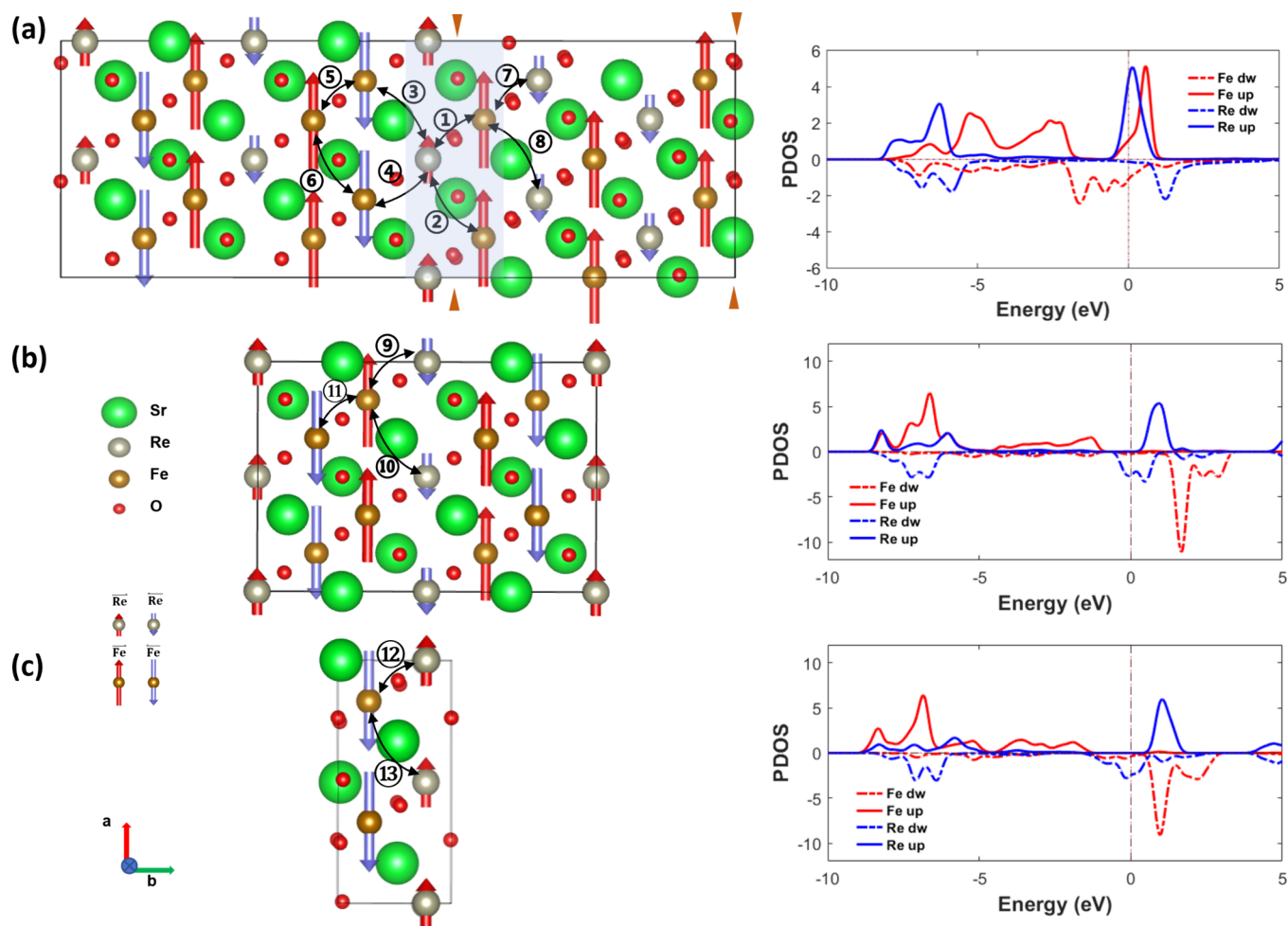
Figure 4. Atomic structure and magnetic coupling of (a) \text{Sr}_3[\text{Fe}]_{\text{B}_1}[\text{Fe}]_{\text{B}_2}[\text{Re}]_{\text{B}_3}\text{O}_9/\text{Sr}_2[\text{Fe}]_{\text{B}_1}[\text{Re}]_{\text{B}_2}\text{O}_6 interface model with the interface indicated by orange triangles, (b) \text{Sr}_3[\text{Fe}]_{\text{B}_1}[\text{Fe}]_{\text{B}_2}[\text{Re}]_{\text{B}_3}\text{O}_9 with the P3m1 space group, and (c) \text{Sr}_2[\text{Fe}]_{\text{B}_1}[\text{Re}]_{\text{B}_2}\text{O}_6 . The atomic structures in panels (a–c) show Sr in green, Re in silver, Fe in gold, and O in red. Spin-down and spin-up magnetic moments are represented by violet and red arrows, respectively. In the right figure in (a), the projected density of states (PDOS) of Fe and Re atoms at the very interface marked by a blue shadow reveals their ferromagnetic coupling, while in the right figures in (b) and (c), the PDOS of adjacent Fe and Re atoms show their antiferromagnetic coupling.
