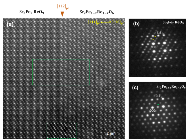
Figure 1. High-angle annular dark-field scanning transmission electron microscopy (HAADF STEM) image and nanodiffraction of the \text{Sr}_3\text{Fe}_2\text{ReO}_9/\text{Sr}_2\text{Fe}_{1+x}\text{Re}_{1-x}\text{O}_6 interface. (a) Green solid rectangle indicates the area used for elemental mapping. The inset in the green dashed rectangle shows a simulated HAADF STEM image of the \text{Sr}_3\text{Fe}_2\text{ReO}_9/\text{Sr}_2\text{Fe}_{1+x}\text{Re}_{1-x}\text{O}_6 interface based on the model shown in Figure 4a below. (b,c) Nanodiffraction patterns recorded from the 1:2 B-site-ordered \text{Sr}_3\text{Fe}_2\text{ReO}_9 phase and the 1:1 B-site-ordered \text{Sr}_2\text{Fe}_{1+x}\text{Re}_{1-x}\text{O}_6 phase, respectively. Fractional super-reflection spots (such as \frac{1}{3}\{111\}_{\text{pc}} , \frac{2}{3}\{111\}_{\text{pc}} ) and half-integer super-reflection spots (such as \frac{1}{2}\{111\}_{\text{pc}} ) are marked by yellow triangles in (b) and green triangles in (c), respectively.
