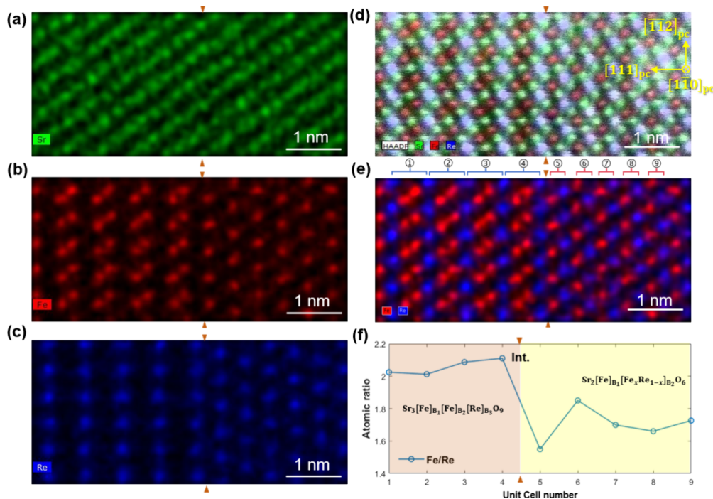
Figure 2. Atomic-resolution elemental mapping of the \text{Sr}_3[\text{Fe}]_{\text{B}_1}[\text{Fe}]_{\text{B}_2}[\text{Re}]_{\text{B}_3}\text{O}_9/\text{Sr}_2[\text{Fe}]_{\text{B}_1}[\text{Fe}_{1/6}\text{Re}_{5/6}]_{\text{B}_2}\text{O}_6 interface, showing (a) Sr in green, (b) Fe in red, (c) Re in blue, (d) elemental mixed Sr, Fe, and Re mapping as well as the HAADF STEM image, and (e) elemental mixed Fe and Re mapping. (f) Statistical Fe/Re ratios of the B-site transition metals on a unit cell by unit cell basis. On the triple-perovskite \text{Sr}_3[\text{Fe}]_{\text{B}_1}[\text{Fe}]_{\text{B}_2}[\text{Re}]_{\text{B}_3}\text{O}_9 side, the unit cell is -\text{[Re-Fe-Fe]}- , while on the double-perovskite \text{Sr}_2[\text{Fe}]_{\text{B}_1}[\text{Fe}_x\text{Re}_{1-x}]_{\text{B}_2}\text{O}_6 side, the nominal 1:1 unit cell is -\text{[Fe-Re]}- . For clarity, the unit number in (e) corresponds to that in (f), and the interface position is indicated by a pair of orange triangles.
