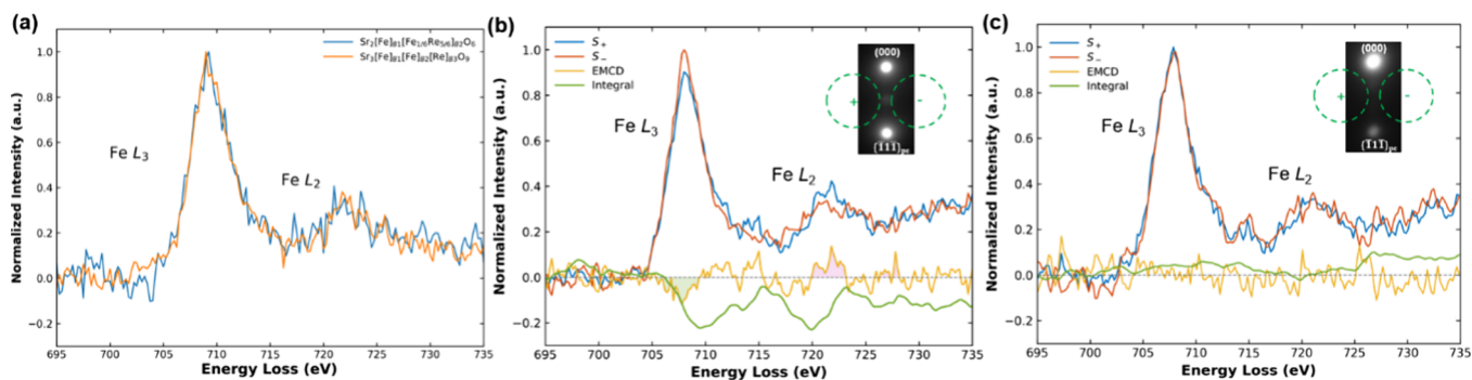
Figure 3. (a) Electron energy-loss (EEL) near-edge fine structures of the Fe L_{3,2} -edges acquired from the double- and triple-perovskite regions and used for Fe-valence assessment. Normalized EEL spectra acquired at the positive “ S_+ ” (blue) and negative “ S_- ” (orange) positions from (b) double-perovskite \text{Sr}_2[\text{Fe}]_{\text{B}_1}[\text{Fe}_{1/6}\text{Re}_{5/6}]_{\text{B}_2}\text{O}_6 and (c) triple-perovskite \text{Sr}_3[\text{Fe}]_{\text{B}_1}[\text{Fe}]_{\text{B}_2}[\text{Re}]_{\text{B}_3}\text{O}_9 regions, respectively. The yellow lines show the electron magnetic circular dichroism (EMCD) spectra. The green lines show the cumulative integral of the residual-baseline-corrected difference spectrum. The insets were recorded under two-beam conditions, where \{\bar{1}\bar{1}\bar{1}\}_{\text{pc}} systematic reflections were excited with an electron probe.
